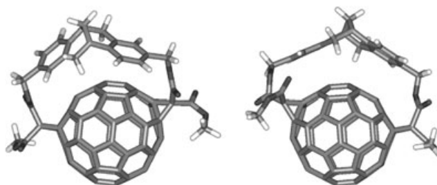
Figure 4. Energy-minimized structures of (S,S,\text{f}^sA) - 9 (left) and (S,S,\text{f}^sC) - 9 (right). Ethyl esters have been substituted by methyl esters for clarity.
