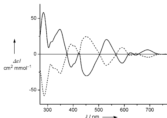
Figure 6. CD spectra of (\text{ᶠ}^{\text{S}}C) (solid line) and (\text{ᶠ}^{\text{S}}A) (dashed line) configured fullerene chromophores with trans -3 addition pattern, obtained by subtraction of the CD spectrum of (R,R)\text{-22} from the spectra of (R,R,\text{ᶠ}^{\text{S}}C)\text{-23a} and (R,R,\text{ᶠ}^{\text{S}}A)\text{-23a} , respectively.
