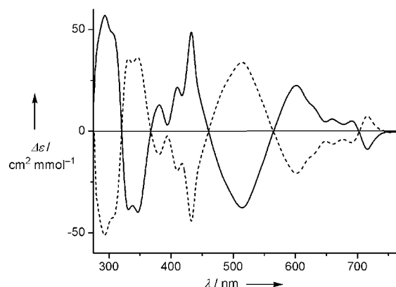
Figure 3. CD spectra of (S,S,\text{f}^sA) - 9 (solid line) and (R,R,\text{f}^sC) - 9 (dashed line) in \text{CHCl}_3 .
