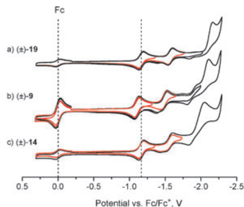
Figure 7. CV of a) 0.2 mM (\pm)\text{-19} , b) 0.2 mM trans -2 (\pm)\text{-9} , and c) 0.2 mM (\pm)\text{-14} in \text{CH}_2\text{Cl}_2 , 0.1 M \text{Bu}_4\text{NPF}_6 , scan rate 100 \text{ mV s}^{-1} , room temperature.
