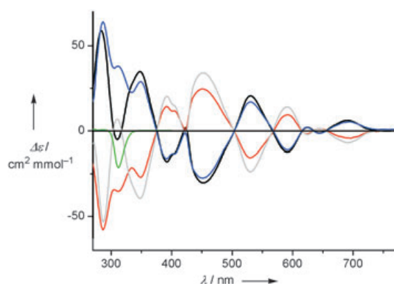
Figure 5. CD spectra of (R,R,\text{ᶠ}^{\text{S}}C)\text{-23a} (black), (R,R,\text{ᶠ}^{\text{S}}A)\text{-23a} (red), (S,S,\text{ᶠ}^{\text{S}}A)\text{-23b} (gray), (S,S,\text{ᶠ}^{\text{S}}C)\text{-23b} (blue), and (R,R)\text{-22} (green) in \text{CHCl}_3 .
